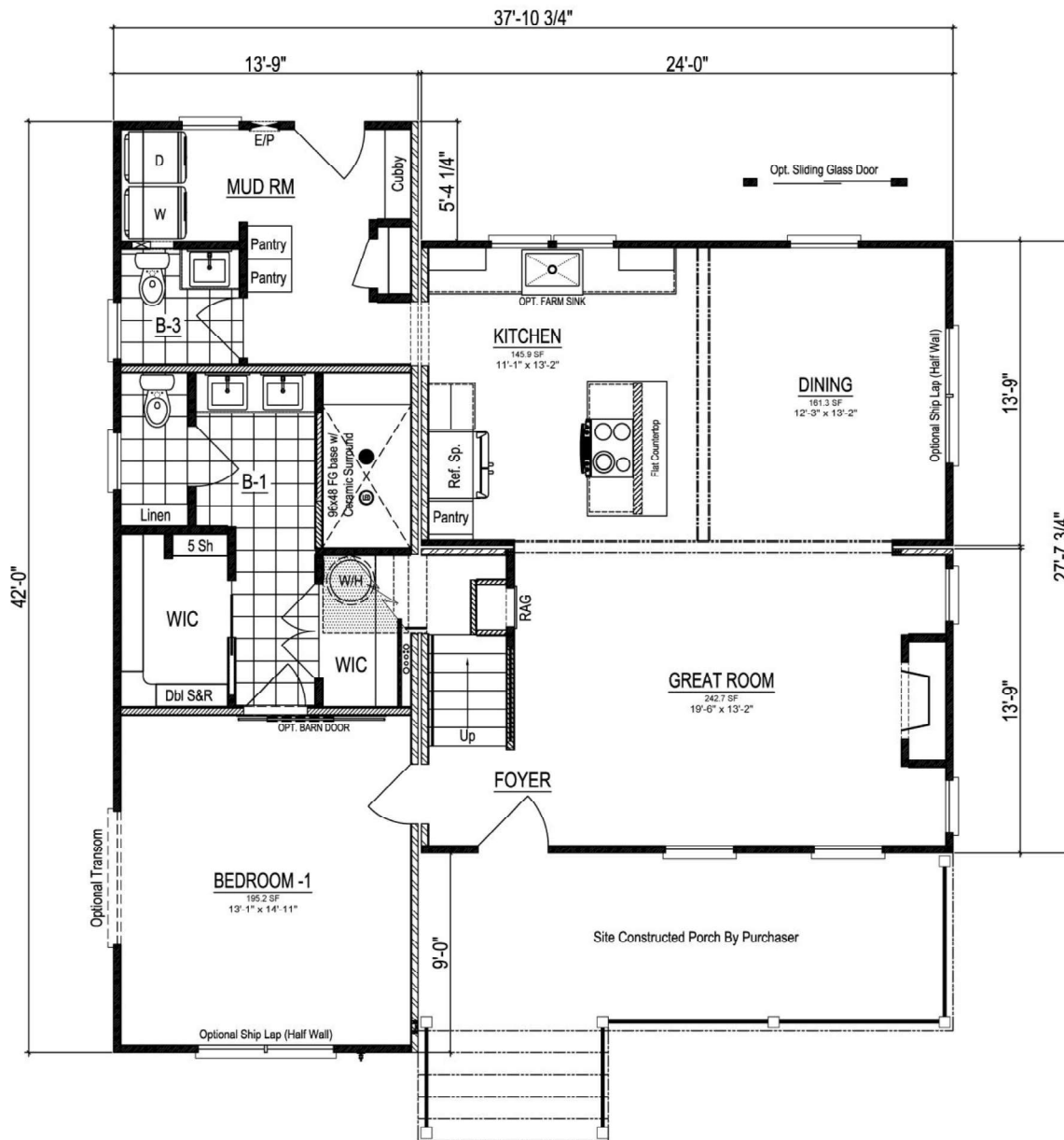
Optional Kitchen Layout
